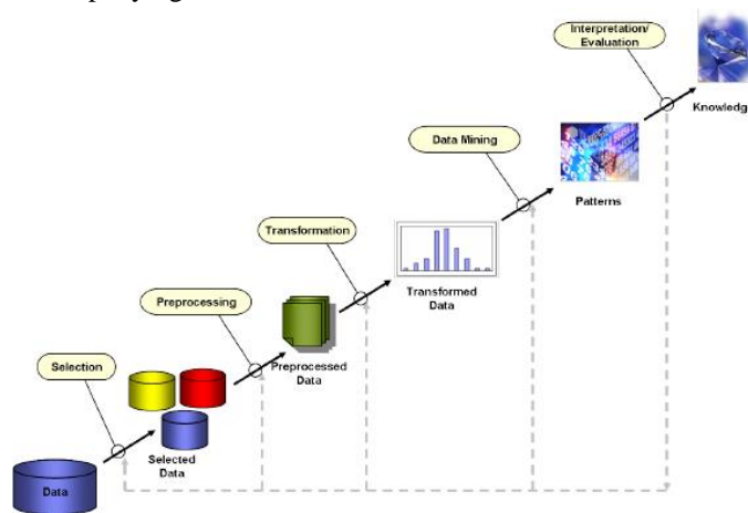
Fig 2: KDD Process
