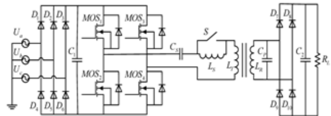
Fig.1: Circuit diagram
