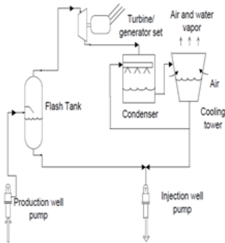
Fig. 1: Example flash-steam geothermal power plant.
