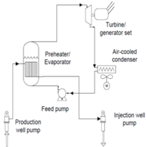
Fig. 2: Example binary-cycle geothermal power plant.
