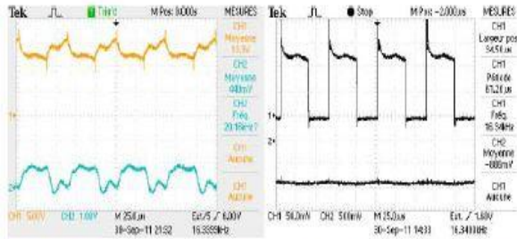
Figure 8. The output voltage and output current respectively from PV at time T3 during the day P=35.92W
