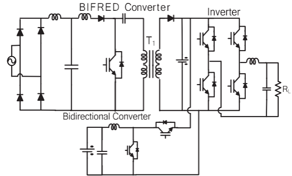
Fig. 3: - UPS system with BIFRED Converter
