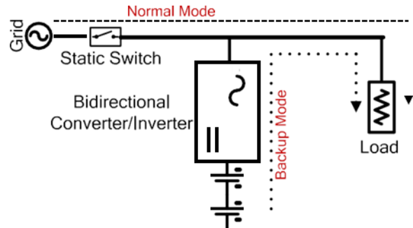
Fig. 2: - Block Diagram of Line Interactive UPS system.
