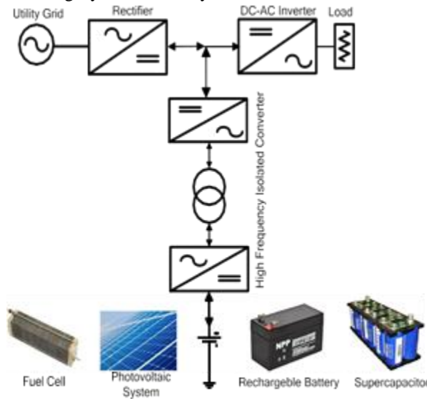
Fig. 4: - Block Diagram of Intelligent UPS system
