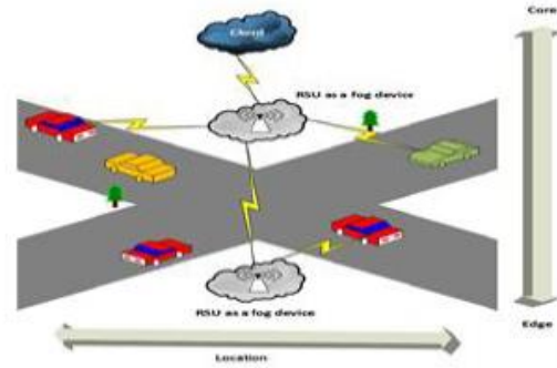
Fig. 4: - Fog based architecture
