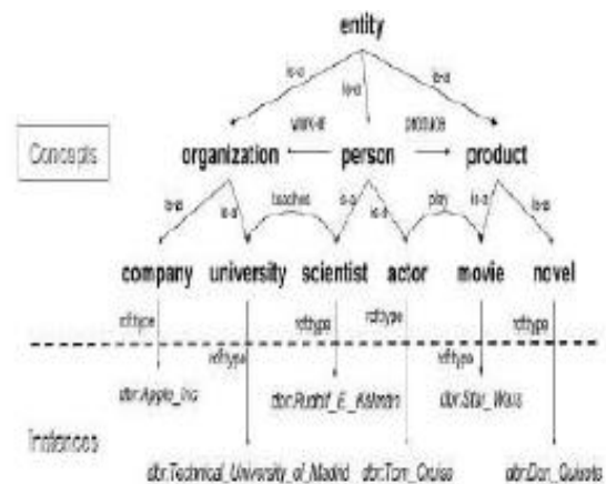
Fig. 1: - Example of knowledge graph.
