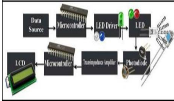
Fig. 8: - Block diagram vehicular Li-Fi
