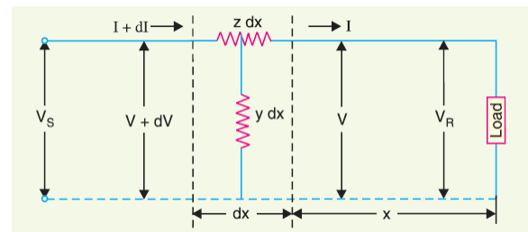
Fig 8 – sectional view of a long transmission line
