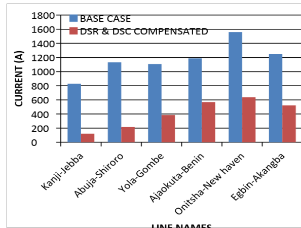
Figure 2; Transmission Line Current Flow Control
