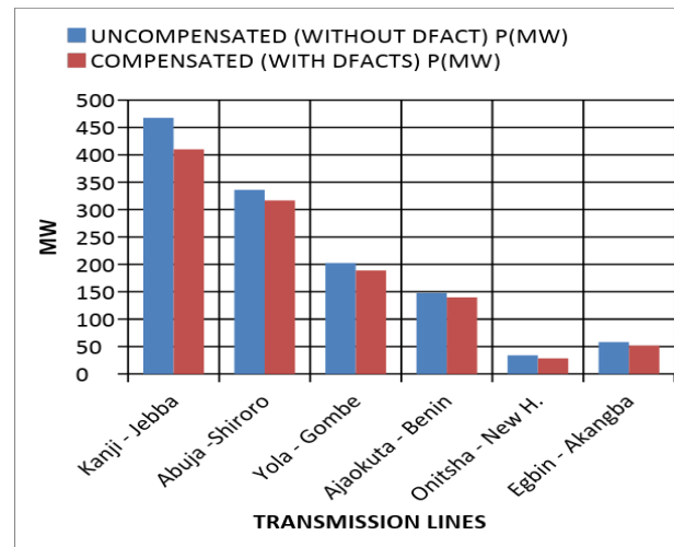
Fig. 3: Real Power flow control without & with D-FACTS compensation
