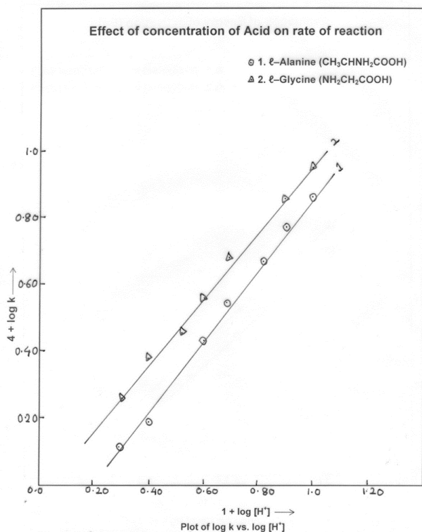
Fig. 1 10^3[\text{DCDMH}] (\text{mol dm}^{-3}) = 2.50 (1, 2) ; 10^2[\text{Substrate}] (\text{mol dm}^{-3}) = 2.00 (1), 1.25 (2) ; \text{HOAc-H}_2\text{O} \% (\text{v/v}) = 30(1), 1.25 (2) ; \text{Temp. K} = 303 (1), 308 (2)
