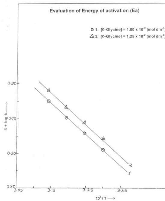
Fig. III-16 [\text{DCDMH}] = 2.50 \times 10^{-3} (\text{mol dm}^{-3}) ; [\text{H}^+] = 0.50 (\text{mol dm}^{-3}) ; \text{HOAc-H}_2\text{O} = 20 \% (\text{v/v})
