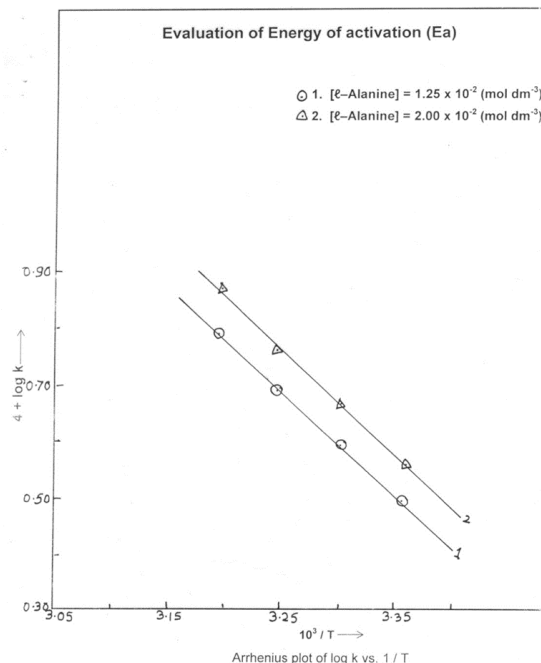
Fig. III-15 [\text{DCDMH}] = 2.50 \times 10^{-3} (\text{mol dm}^{-3}) ; [\text{H}^+] = 0.66 (\text{mol dm}^{-3}) ; \text{HOAc-H}_2\text{O} = 30 \% (\text{v/v})
