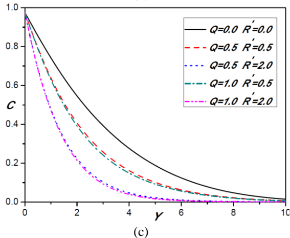
Fig-3.2: Effect of heat generation and chemical reaction parameters on (a) Velocity, (b) Temperature and (c) Concentration profiles at X=1 .
