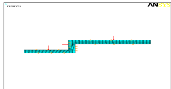
Figure: Boundary conditions for steady state and transient analysis
