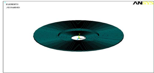
Figure: Full geometry of brake drum with elements
