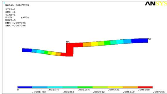
Figure: Thermal deformation for cast iron material
