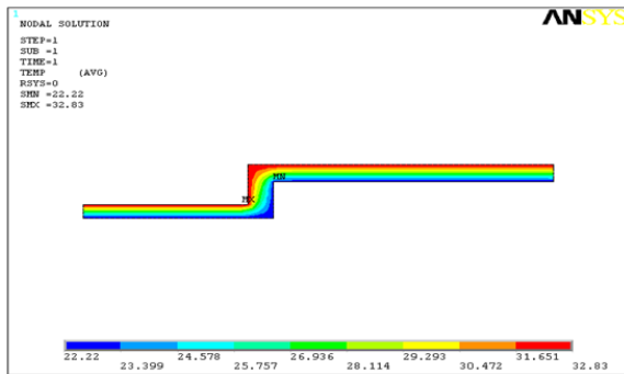
Figure: Temperature distribution for aluminum composite material in steady state condition
