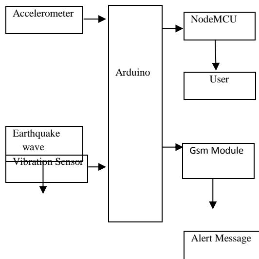
Figure 2.1 Block Diagram of the Proposed System
