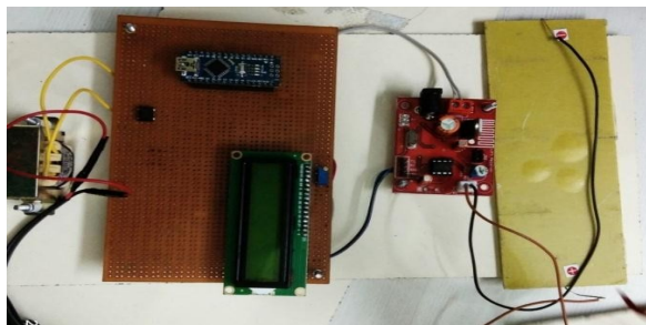
Fig. 8: Receiver Section
