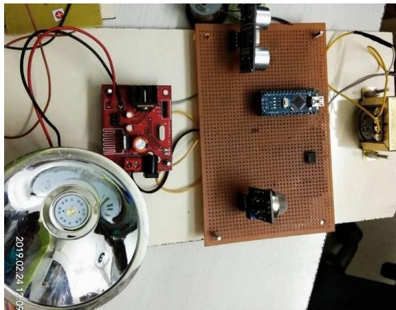
Fig. 7: Transmitter section
