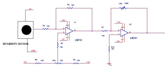
Fig.4 Humidity sensor
