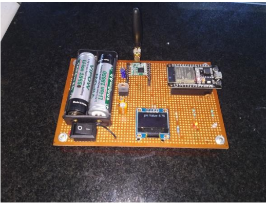
Fig.4. Experimental setup of Gateway node
