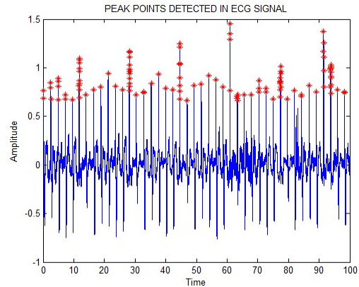
Fig. 4: Peak points detection
