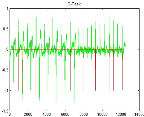
Fig. 4.3: Q - Peak Detection
