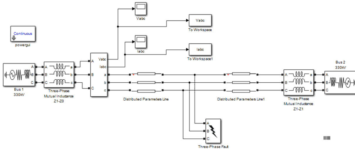
Figure 7: Simulation Model of Faulted Three-Phase Transmission Line
