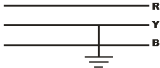
Figure 4: Double Line-to-Ground Fault
