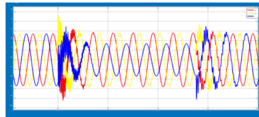
Figure 12: L-G Voltage Waveform (Phase C).
