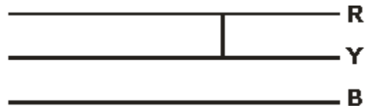
Figure 3: Line-to-Line Fault
