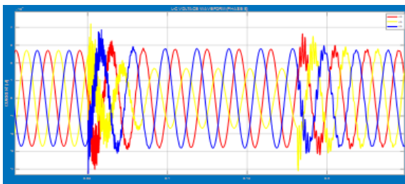
Figure 10: L-G Voltage Waveform (Phase B).
