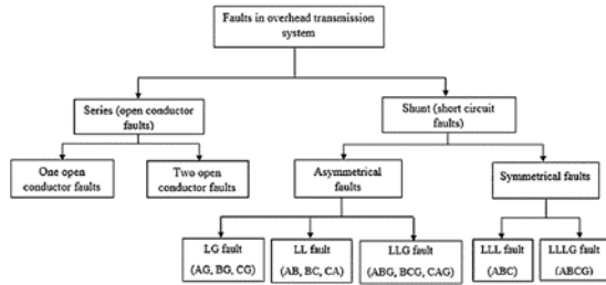
Figure 1: Classification of Faults
