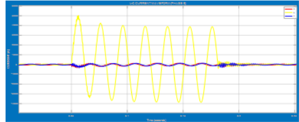
Figure 11: L-G Current Waveform (Phase B).
