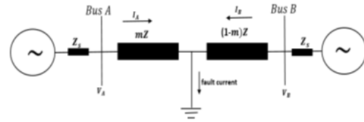
Figure 6: Faulted Three-phase Transmission Line
