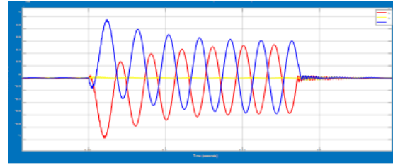
Figure 17: L-L-G Current Waveform (Phase A and C).
