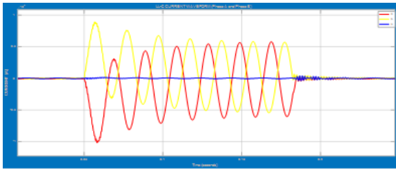
Figure 15: L-L-G Current Waveform (Phase A and B).
