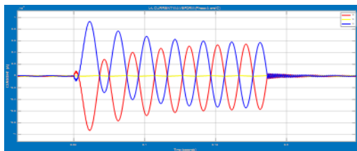
Figure 23: L-L Current Waveform (Phase A and C).
