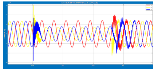
Figure 18: L-L-G Voltage Waveform (Phase B and C).
