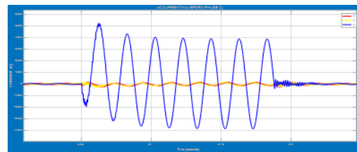
Figure 13: L-G Current Waveform (Phase C).
