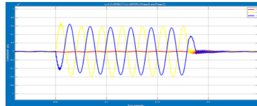
Figure 19: L-L-G Current Waveform (Phase B and C).
