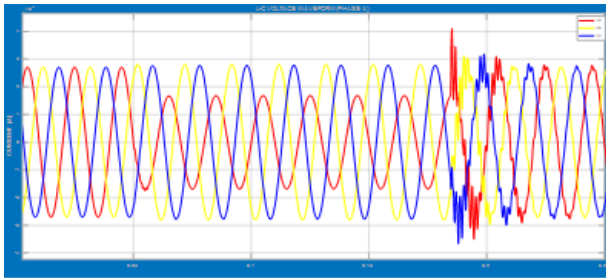
Figure 8: L-G Voltage Waveform (Phase A).
