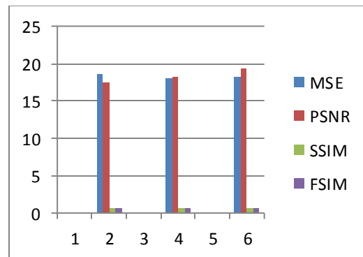
Chart 2: MSE, PSNR, SSIM and PSNR values for Gaussian Noise Variance 0.6
