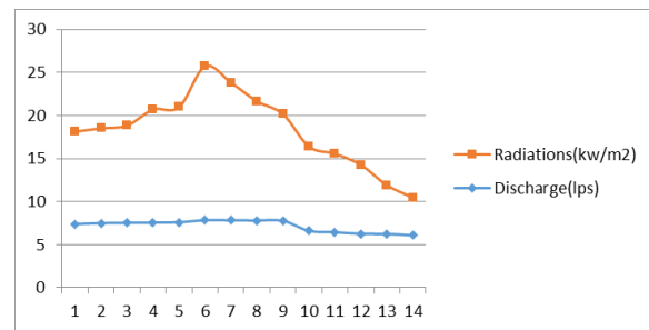
Fig .2: Graphical representation of incident radiation and discharge.
