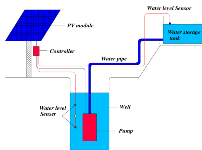
Fig. 1: Schematic view of solar pumping system with PV-Array
