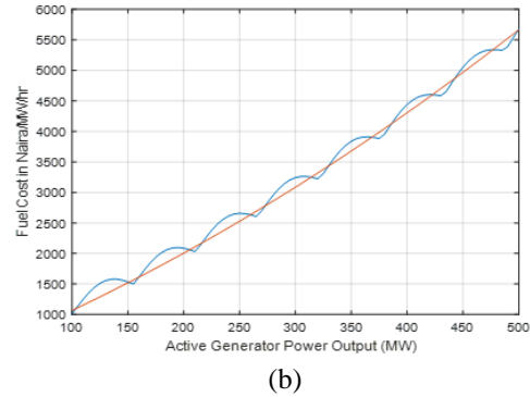
Figure 2: Plot of Cost-Output characteristic for generator at bus 1 (Gen1)
