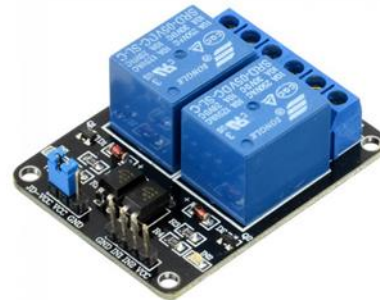
Fig2: Relay module
