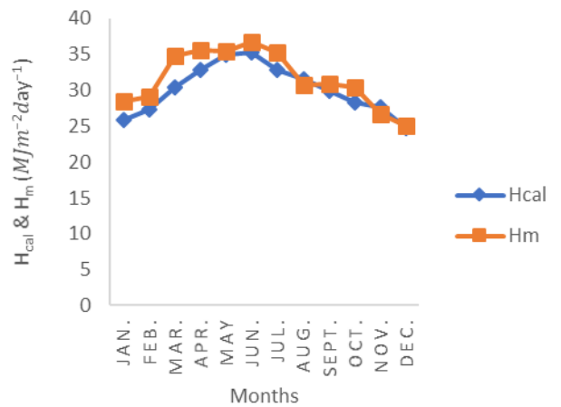
Figure 2: Comparison between measured and calculated value of global solar irradiance
