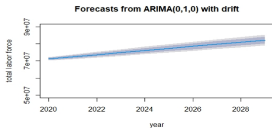
Figure 5. Forecasting for 10 years with upper and lower bounds
