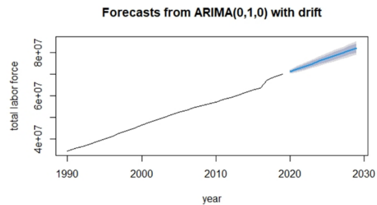
Figure 4. Total labor force forecasting for 10 years
