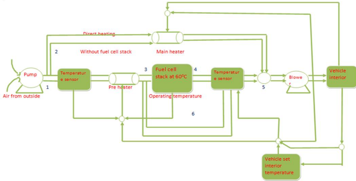
Figure: Heat transfer mechanism showing different components
