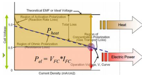
Graph: V-I characteristics of fuel cell
