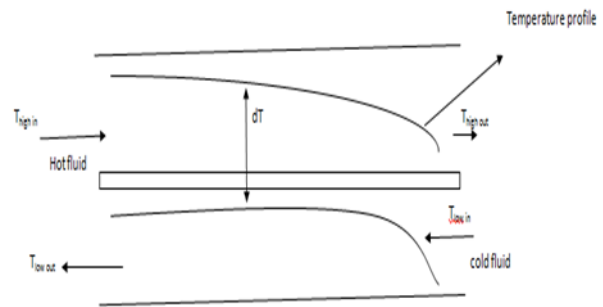
Figure: Temperature profile of hot and cold fluid when flown in opposite direction
