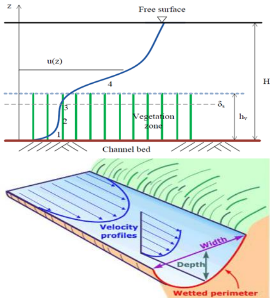
Figure 1; Vertical Velocity Profile of Submerged Vegetation (Baptisetal.2007)
