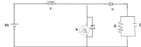
Fig 5: Schematic diagram of boost converter
