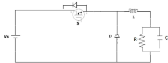
Fig 4: Schematic diagram of buck converter
