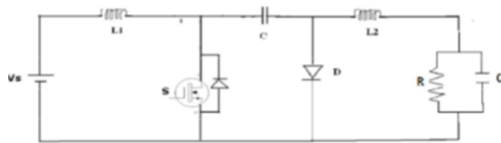
Fig 7: Schematic diagram of cuk converter
