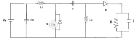
Fig 8: Schematic diagram of SEPIC converter
