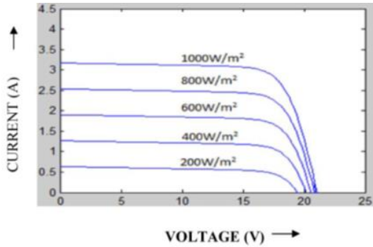
Fig. 2: Current vs Voltage characteristics of PV array
