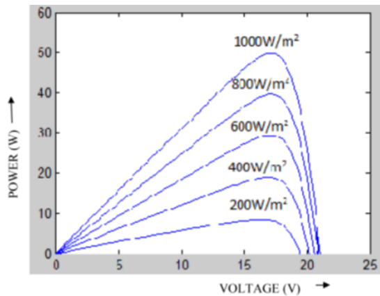
Fig 3: Power vs Voltage characteristics of PV array
