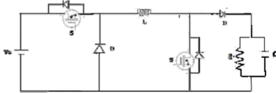
Fig 6: Schematic converter of buck-boost converter.
