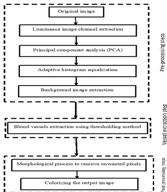
Figure 2. Block diagram of the proposed method
