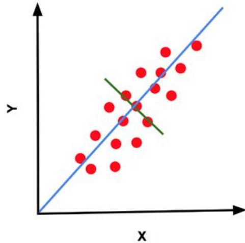
Figure 1. Graphical representation of PCA coordinates
