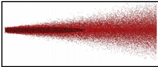
Figure: 12. Heavy flow multi-hole spray flash meshing model
