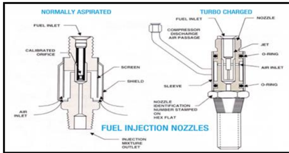
Figure: 3. Fuel inject aero nozzle
