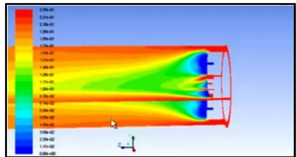
Figure: 21. Counter of mass friction 2
