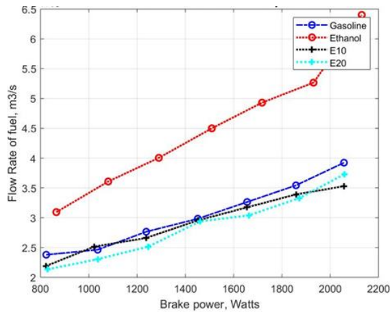
Fig 6. Flow Rate of Fuel Vs Brake Power for compression ratio 8
