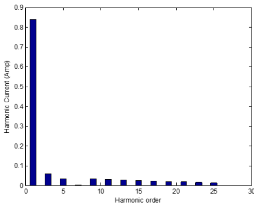
Fig. 11: Harmonic Spectrum of ESL
