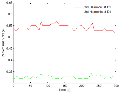
Fig. 4: Comparison of Harmonic pattern at Periods D_1 and D_4
