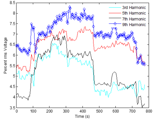
Fig. 6: Comparison of Dominant Harmonic Components with all Loads Connected
