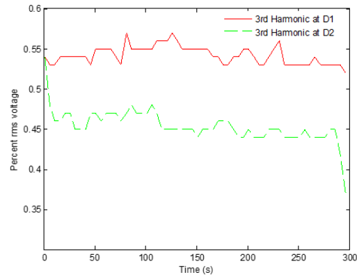
Fig. 2: Comparison of Harmonic pattern at Periods D 1 and D 2
