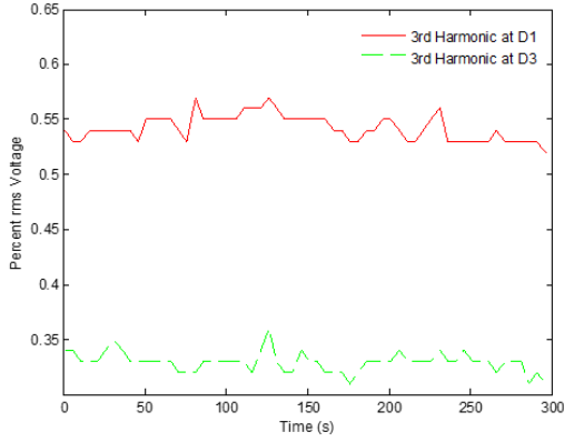
Fig. 3: Comparison of Harmonic pattern at Periods D_1 and D_3
