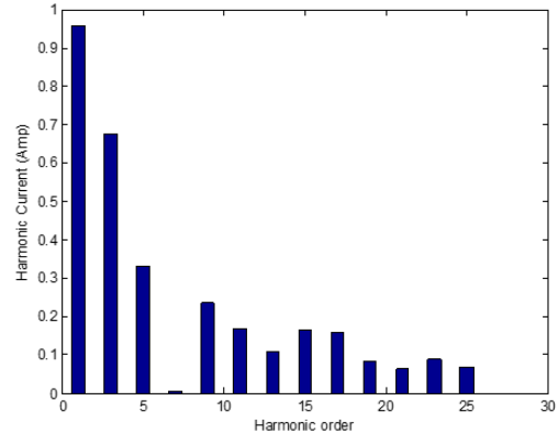
Fig. 12: Harmonic Spectrum of BFL
