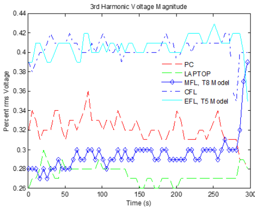
Fig. 5: Comparison of Individual Harmonic patterns
