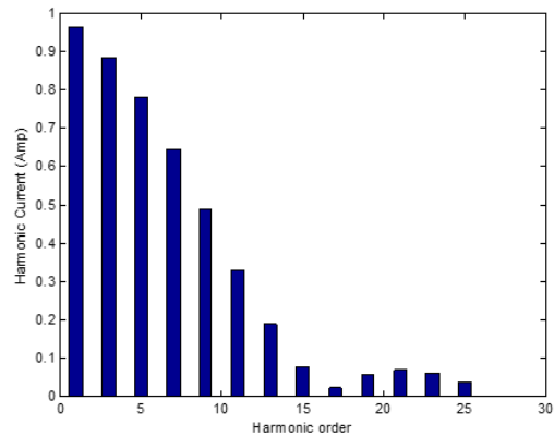
Fig. 8: Harmonic Spectrum of PC
