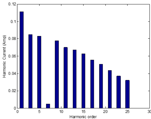
Fig. 10: Harmonic Spectrum of BFL
