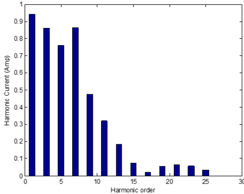
Fig. 9: Harmonic Spectrum of Laptop
