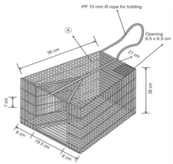
Figure 10a-d: Box trap
