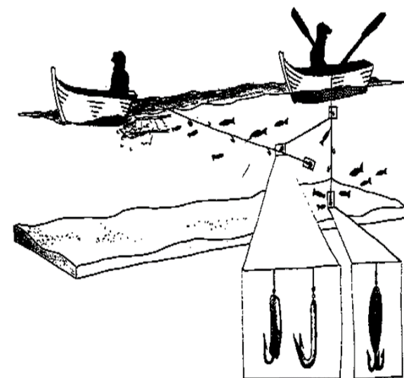
Figure 4: Catching principle and construction of trolling (left) and jigging (right). Expanded view: examples of lures and jig (Dienne and Olopade, 2017).
