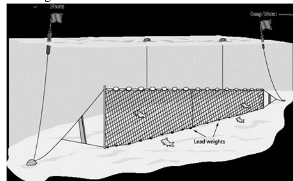
Figure 13c: Set gillnets
