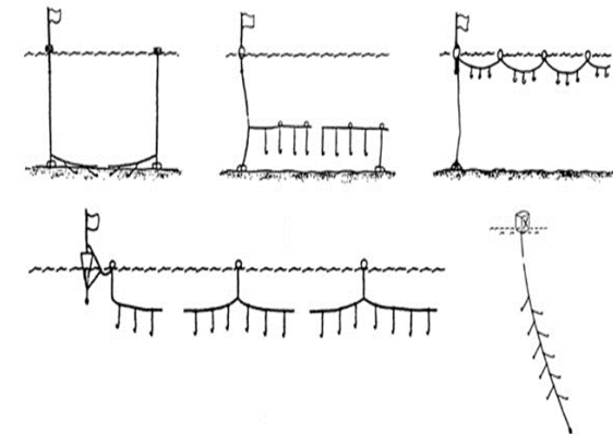
Figure 3: Hooks and Lines fishing gears
