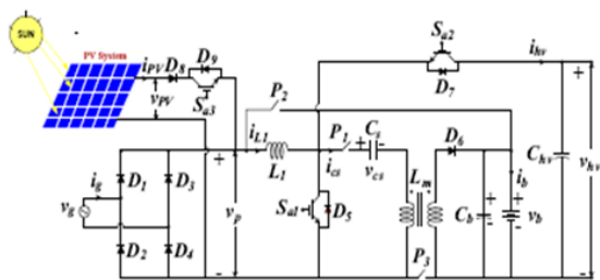
Fig. 3. Configuration of the proposed power conversion system.
