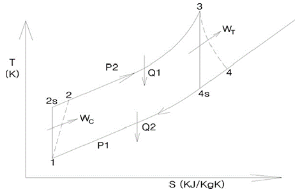
Figure: T – S Diagram for the Simple Gas Turbine Operation [9][10][12][15]
